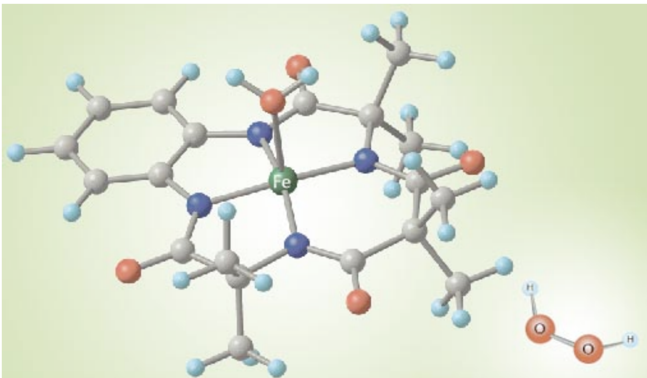
The prototype TAML activator or a relative plus hydrogen peroxide
